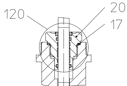
I. EPDM-sealing
